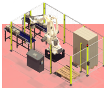
ROBOT ANTROPOMORFO (ARM)
